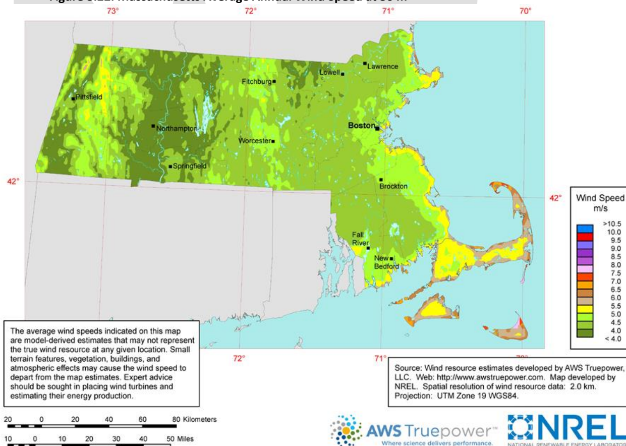
Figure 3.22: Massachusetts Average Annual Wind Speed at 30 m
